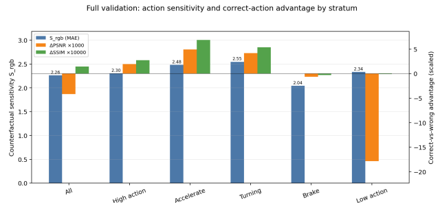
Figure 3. Action sensitivity and correct-action advantage by stratum. The model is most sensitive on turning and acceleration clips, and those same strata show positive correct-vs-wrong PSNR/SSIM advantage.
