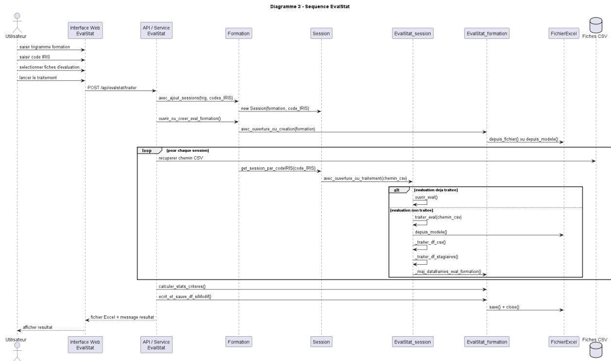
FIGURE 4.1 – Sequence EvalStat
