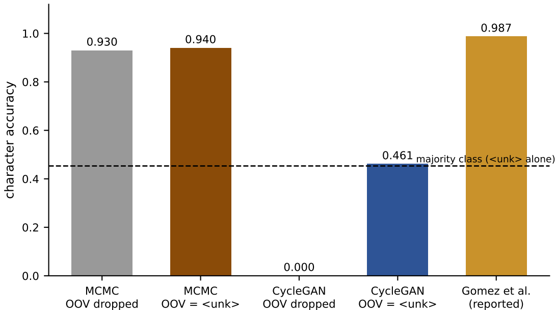
Word-level substitution, 200 types
