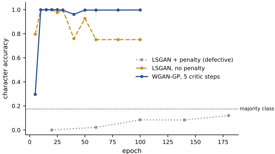
Identity control: locating the objective mis-scaling
