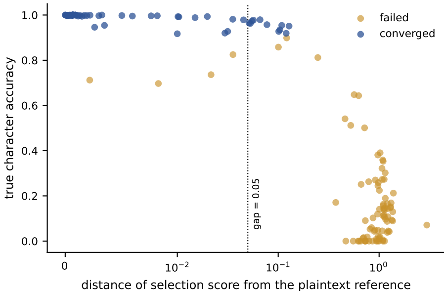
Selection score against true accuracy, all runs
