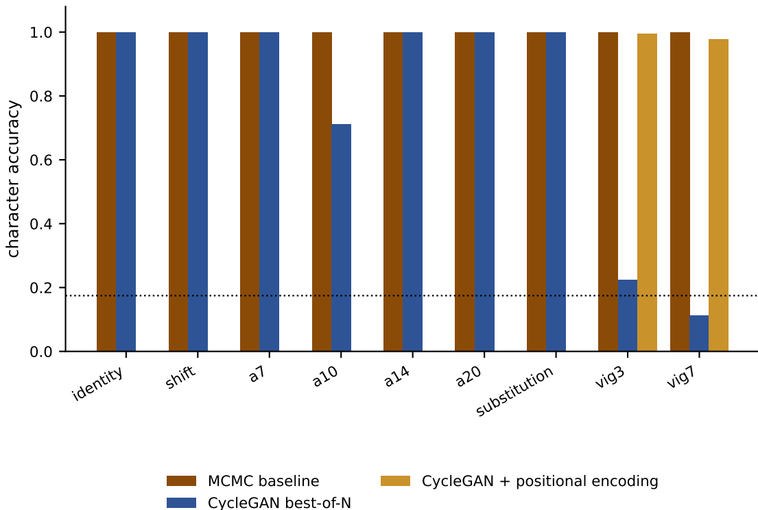
Against a competent classical attack
