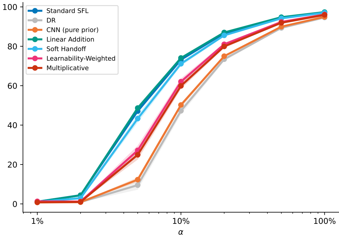
Mean win rate % on worst- \alpha % levels
