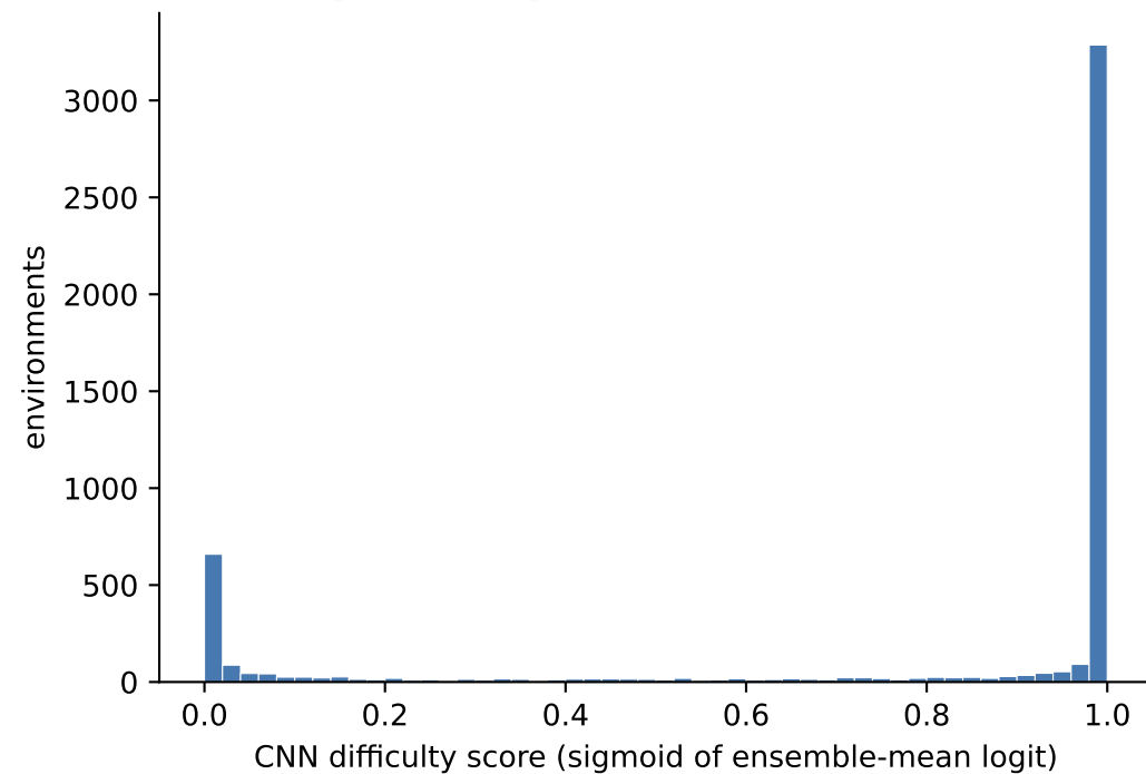
Sigmoid scores of 5000 DR-sampled environments 76.1% outside [0.01, 0.99] (11.9% below 0.01, 64.2% above 0.99)
