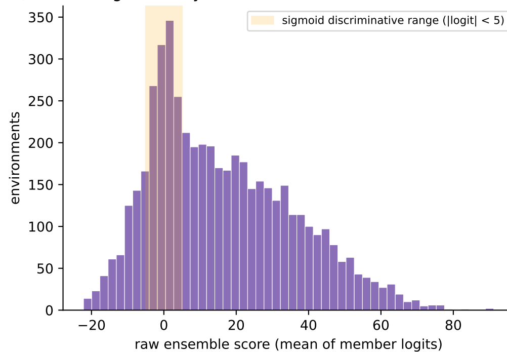
Raw scores span 113 logits; sigmoid only discriminates in the shaded band
