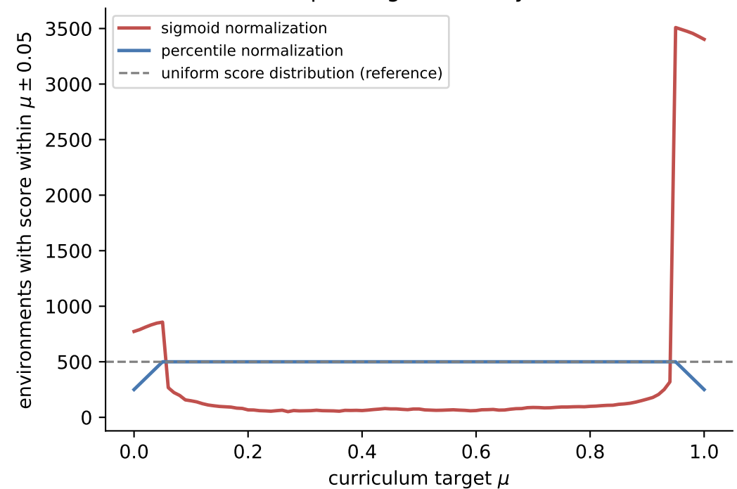
Curriculum coverage: candidates available per target difficulty
