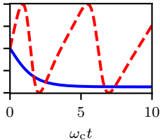
(b) \omega/\omega_c = 0.5
