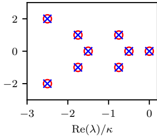
(c) \omega/\omega_c = 50
