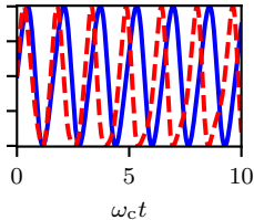
(c) \omega/\omega_c = 4
