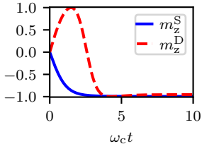
(a) \omega/\omega_c = 0.1
