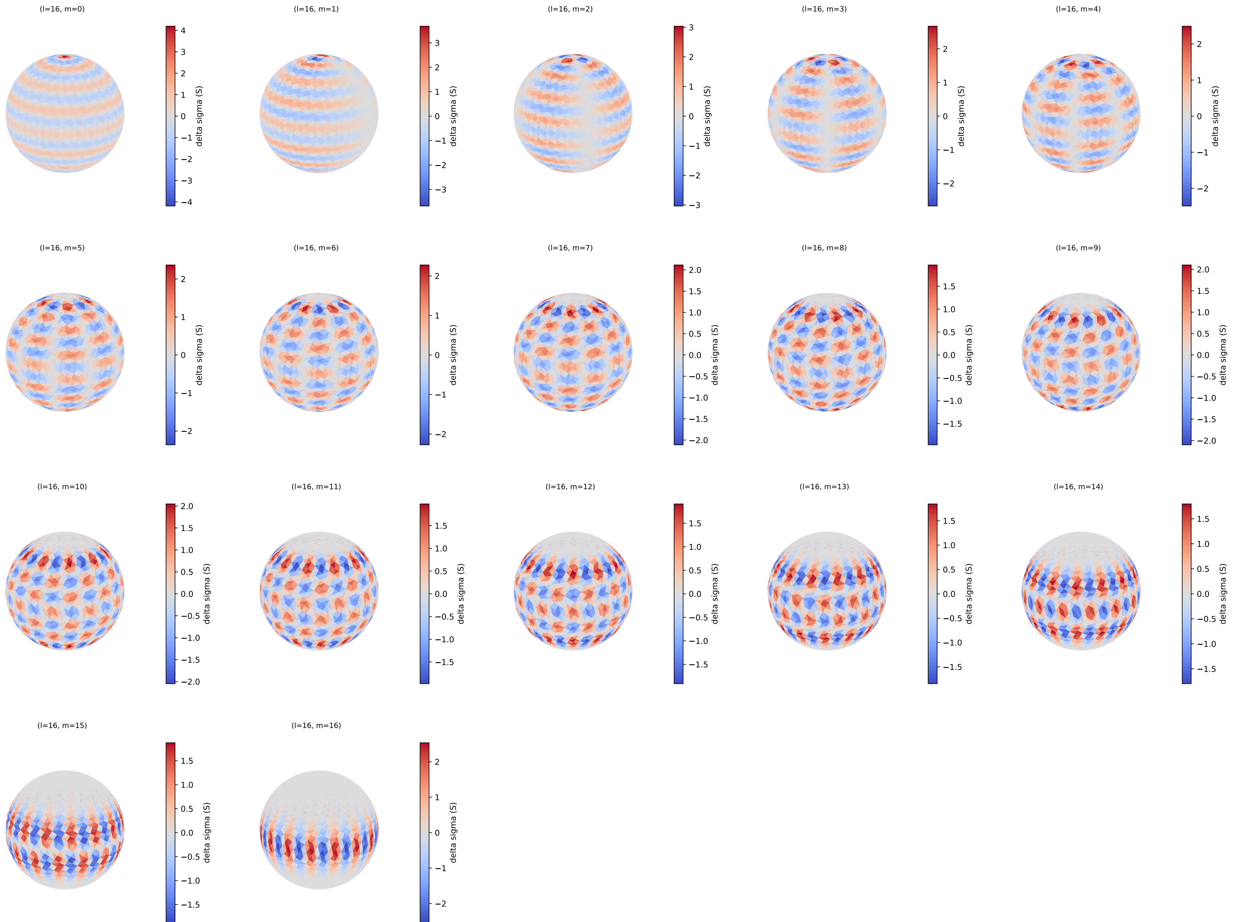
Real Conductivity Harmonics: l=16 , m=0..16 (delta sigma RMS=1.000e+00 S)
