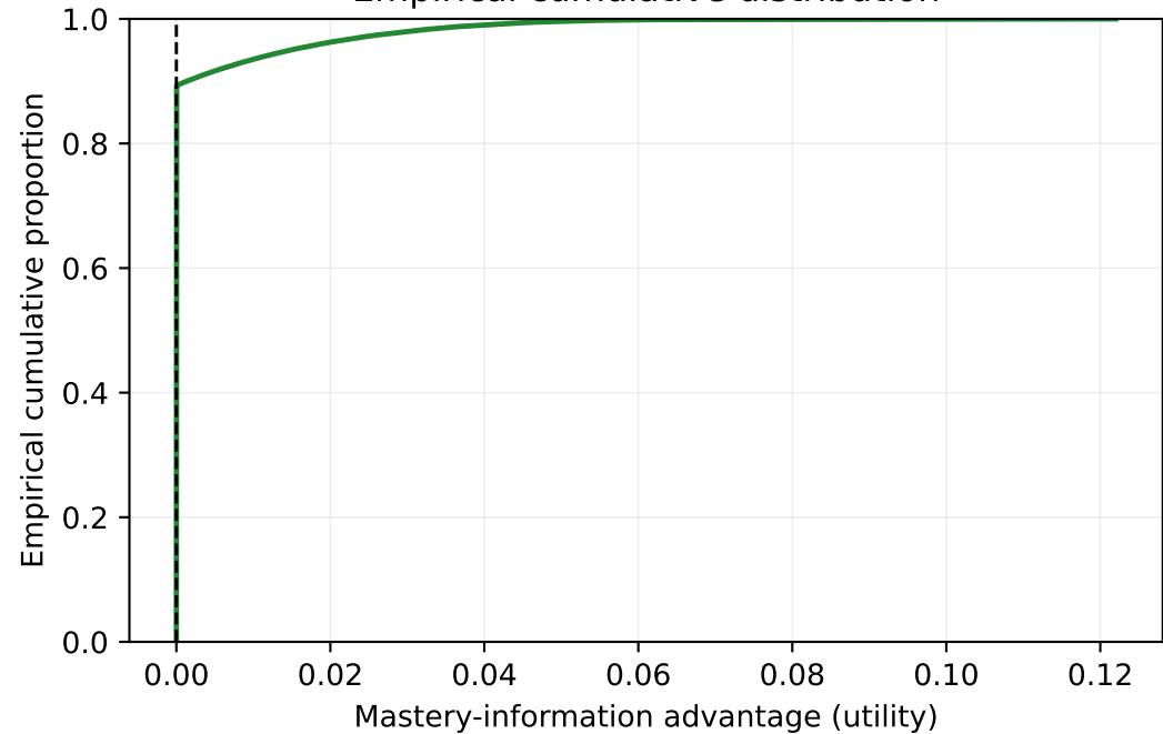
Empirical cumulative distribution
