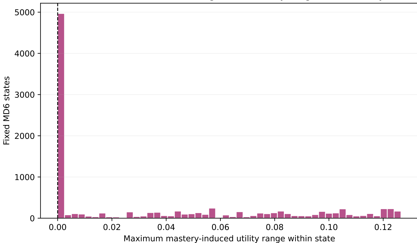
Distribution of maximum eligible-arm utility range over mastery
