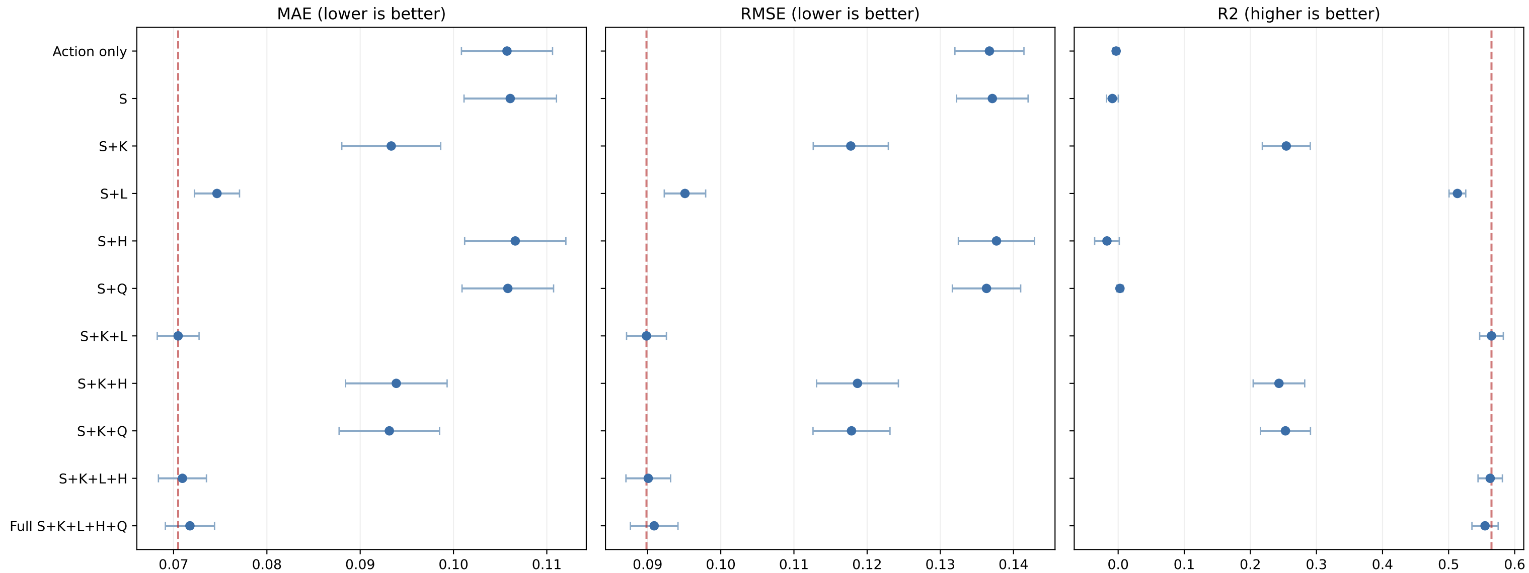
Learner-grouped pre-action context ablation: mean \pm SE across 5 folds
