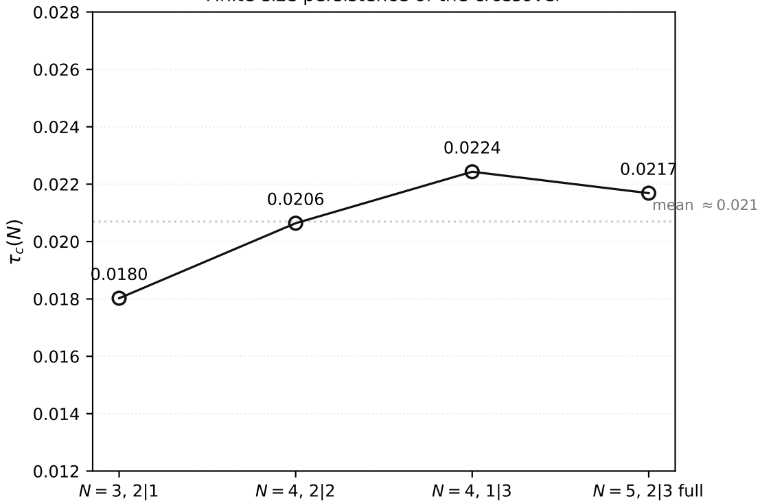
Finite-size persistence of the crossover
