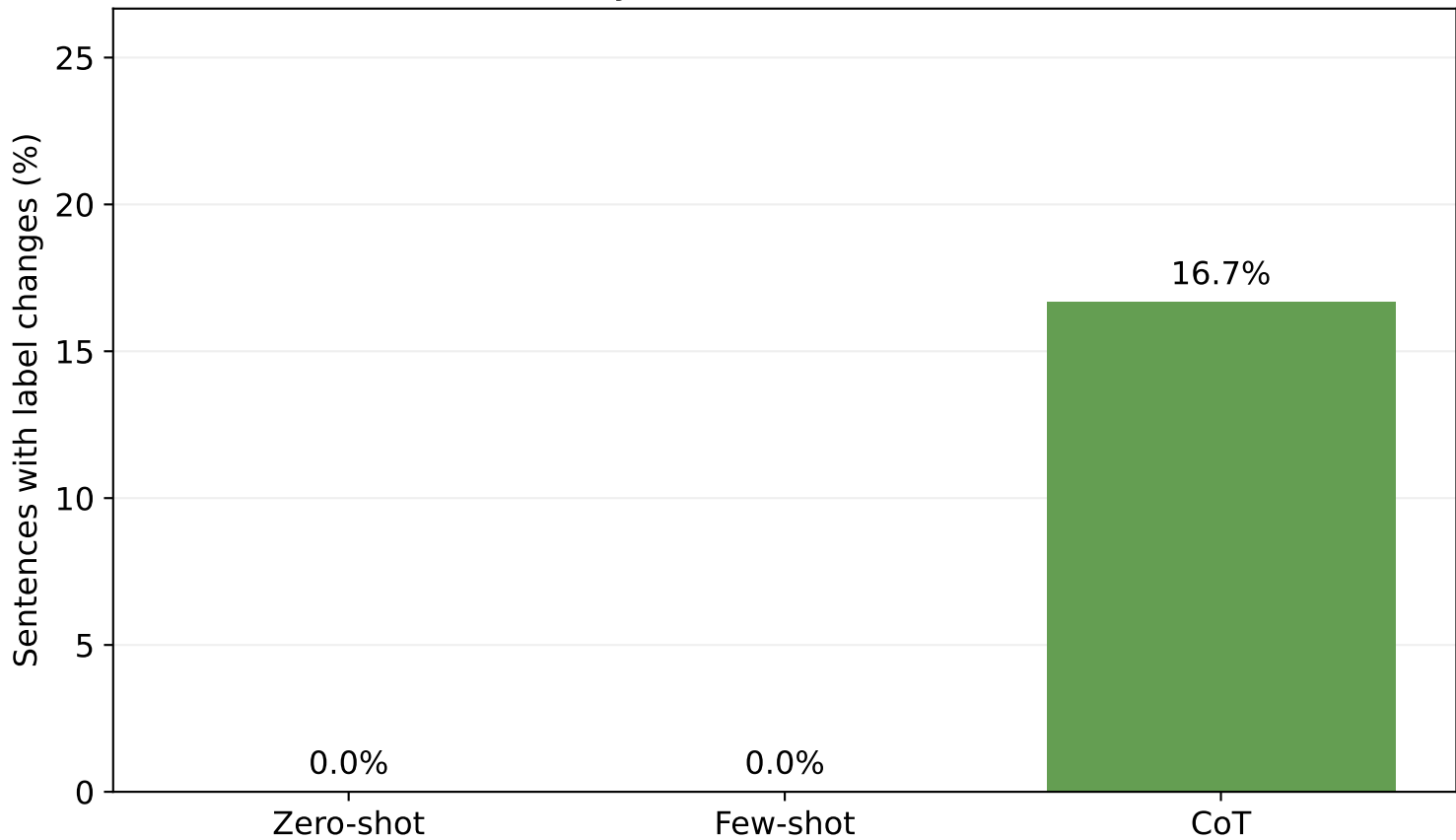
Label instability: 30 sentences, three runs each
