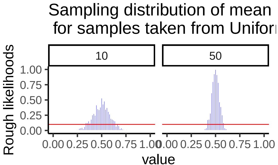
Figure 4.13: Even when samples come from a flat uniform distribution, the distribution of sample means is approximately normal.
