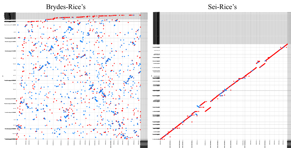
Figure 3. MUMmer plots visualizing the alignment of the Rice's whale genome with that of the Bryde's whale (left) and Sei whale (right). Red segments represent forward matches between the genomes, and blue segments represent reverse matches. Markings on the axes represent the chromosomes of the corresponding genome.
