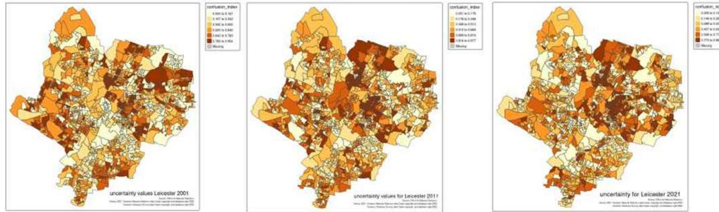
Figure 17 confusion index 2001 , 2011, 2021
