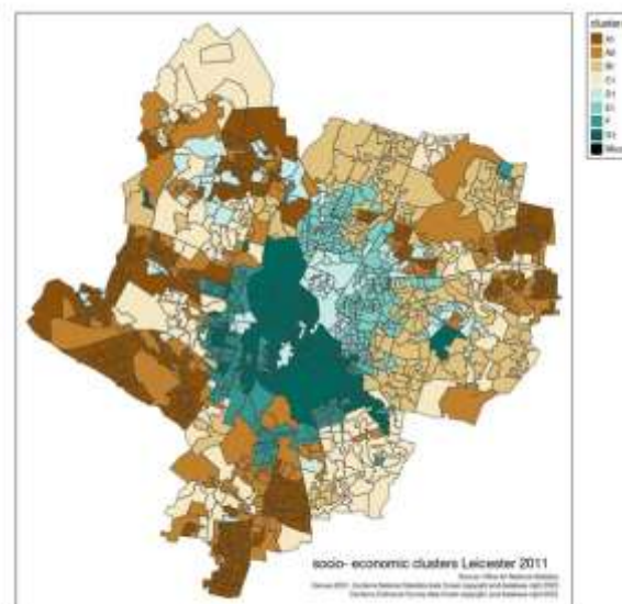
Figure 14 fuzzy c-means classification for 2011
