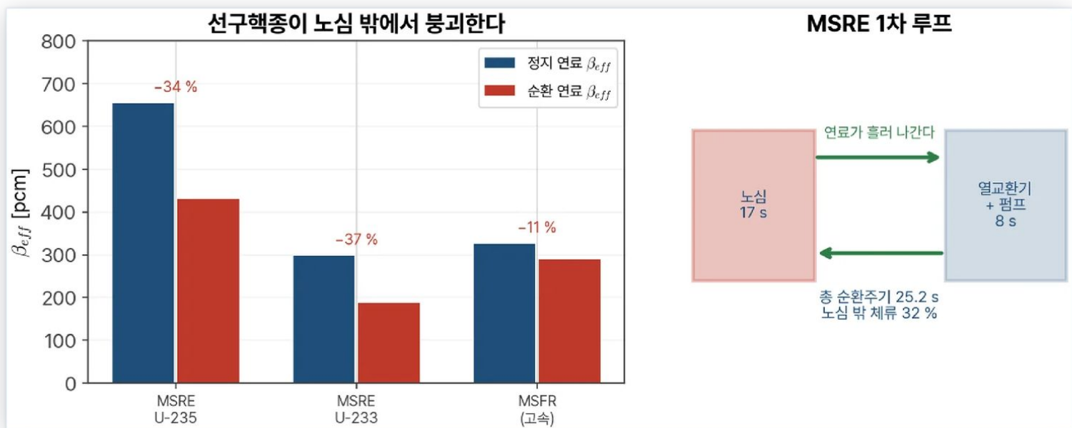
\beta_{eff} reduction from precursor drift (left) and MSRE loop residence times (right) · textbook Fig. 13.1
