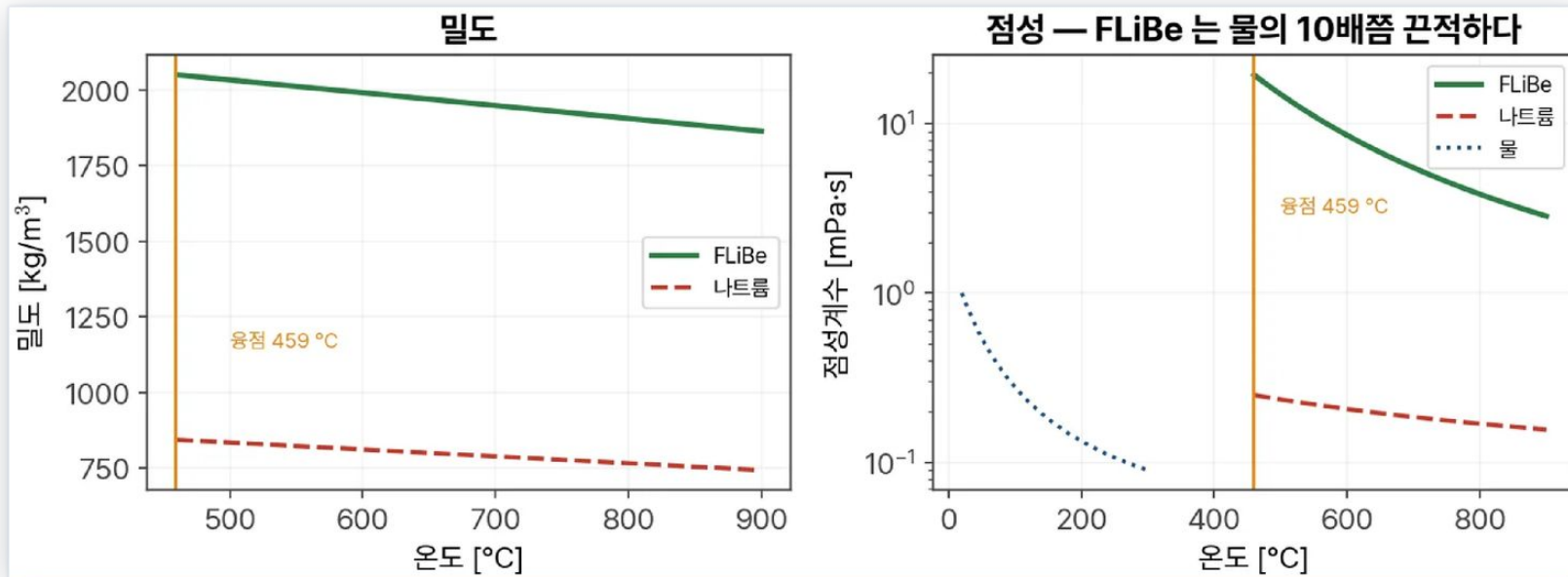
Density and viscosity of FLiBe (solid) and sodium (dashed) - the orange line is the 459 °C FLiBe melting point · textbook Fig. 12.1
