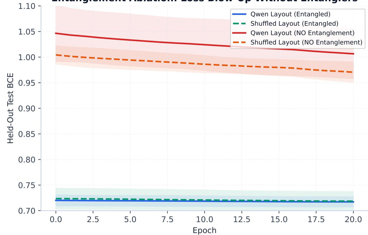
Entanglement Ablation: Loss Blow-Up Without Entanglers
