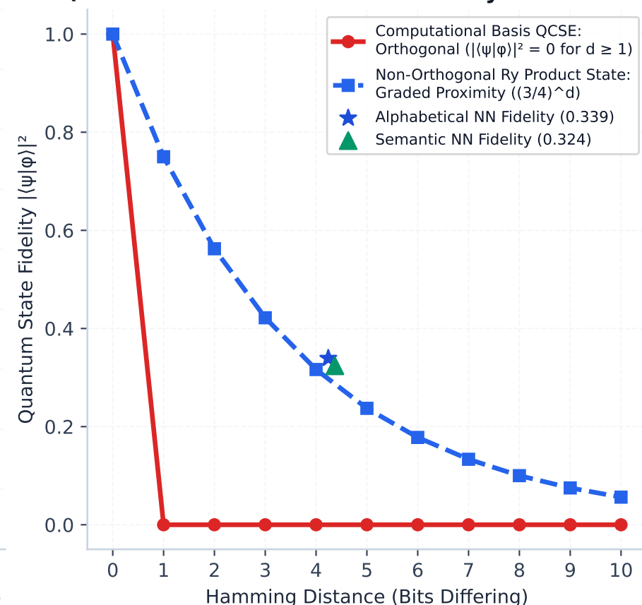
Quantum Proximity vs. Orthogonality (Shared Ansatz Preserves Fidelity: \Delta F < 4e-15 )
