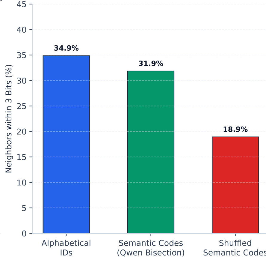
Proportion of Nearest Neighbors within 3-Bit Radius
