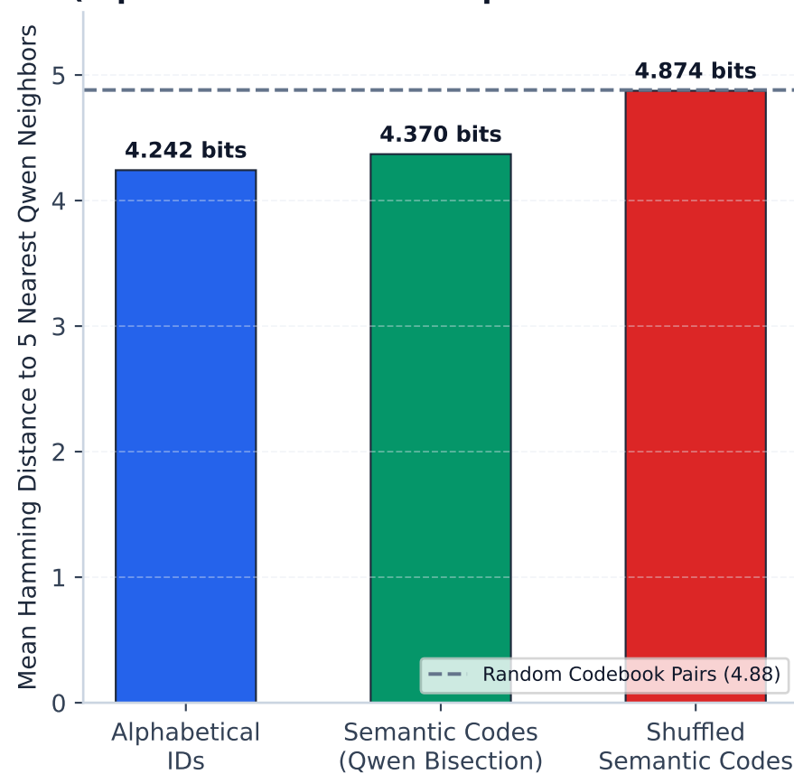
Lexical Codebook Locality (Alphabetical Beats Unsupervised Semantic!)
