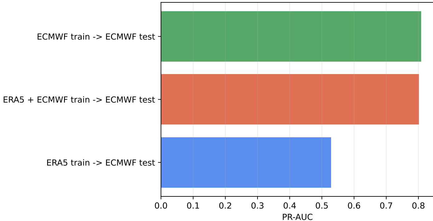
ECMWF Test PR-AUC By Training Source
