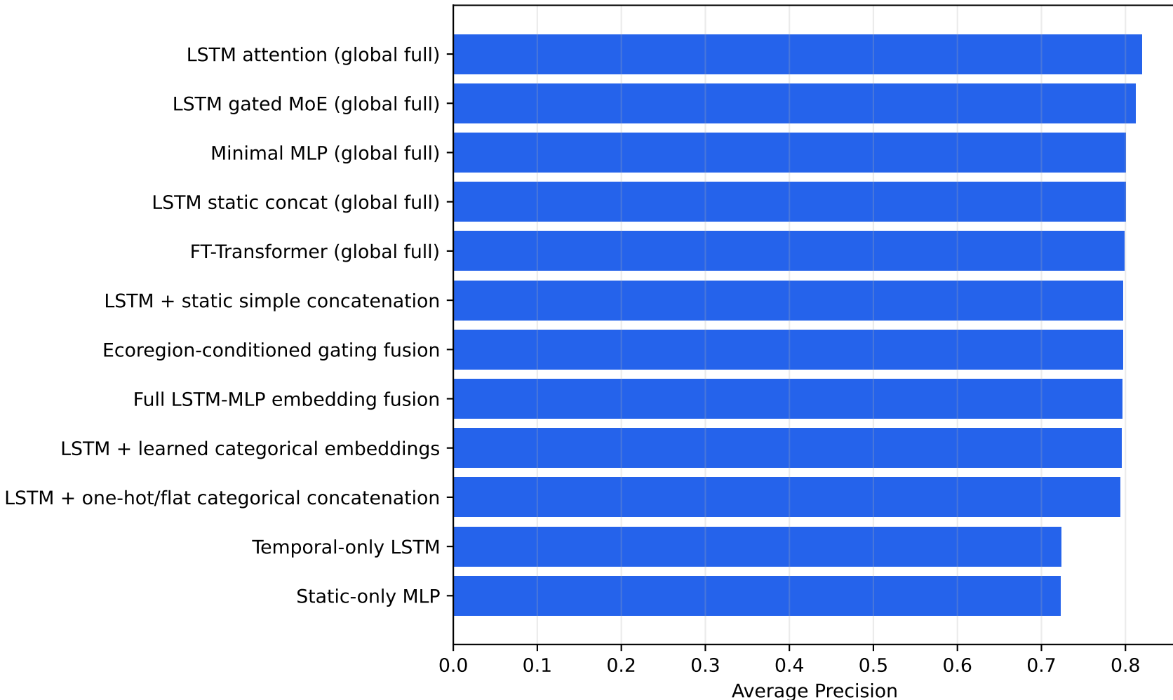
Neural Model / Fusion PR-AUC
