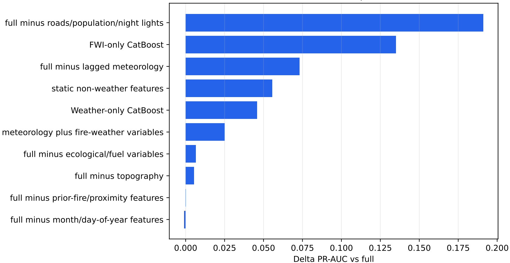
Feature Ablation PR-AUC Drop vs Full CatBoost
