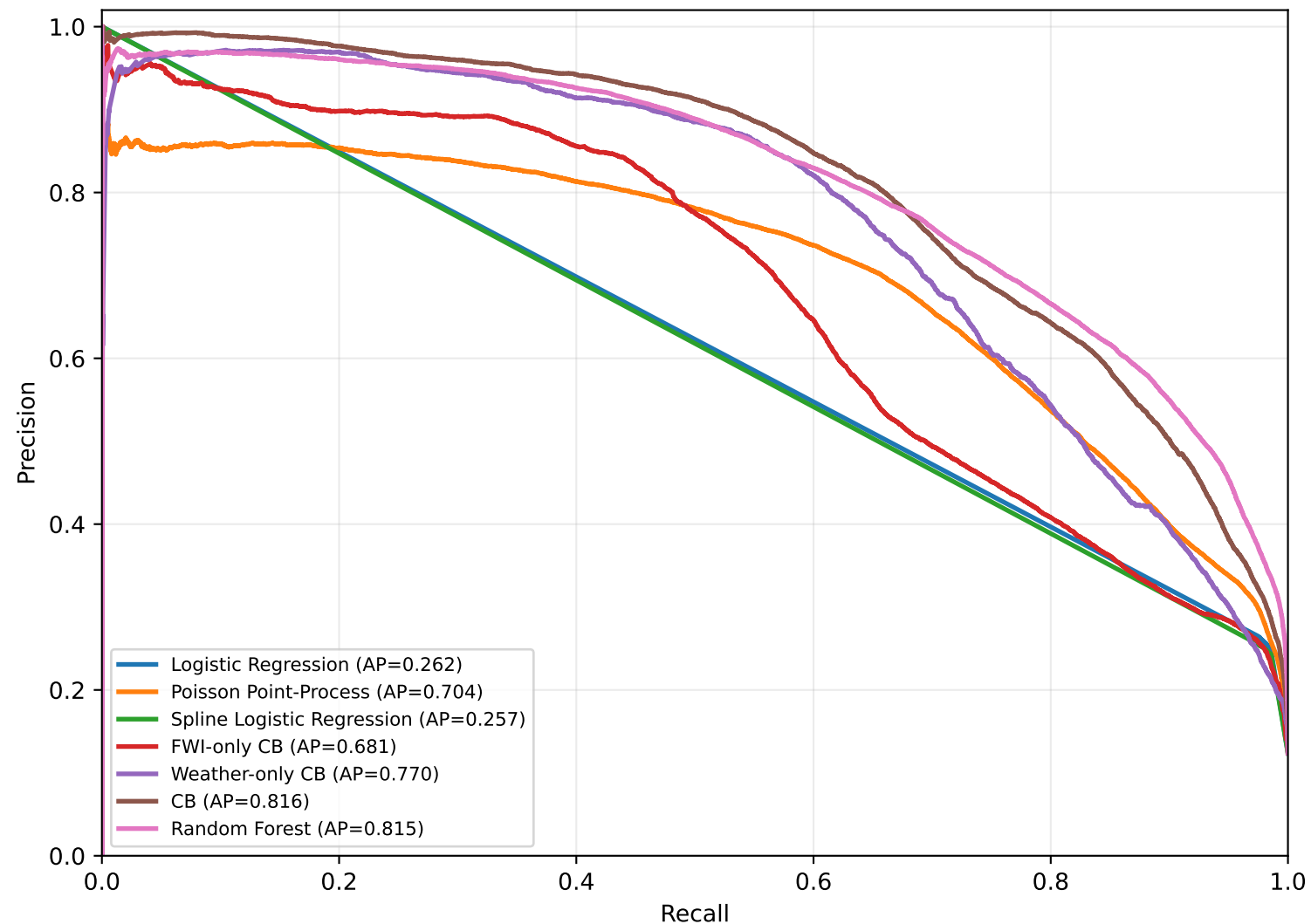
Global Test Precision-Recall Curves
