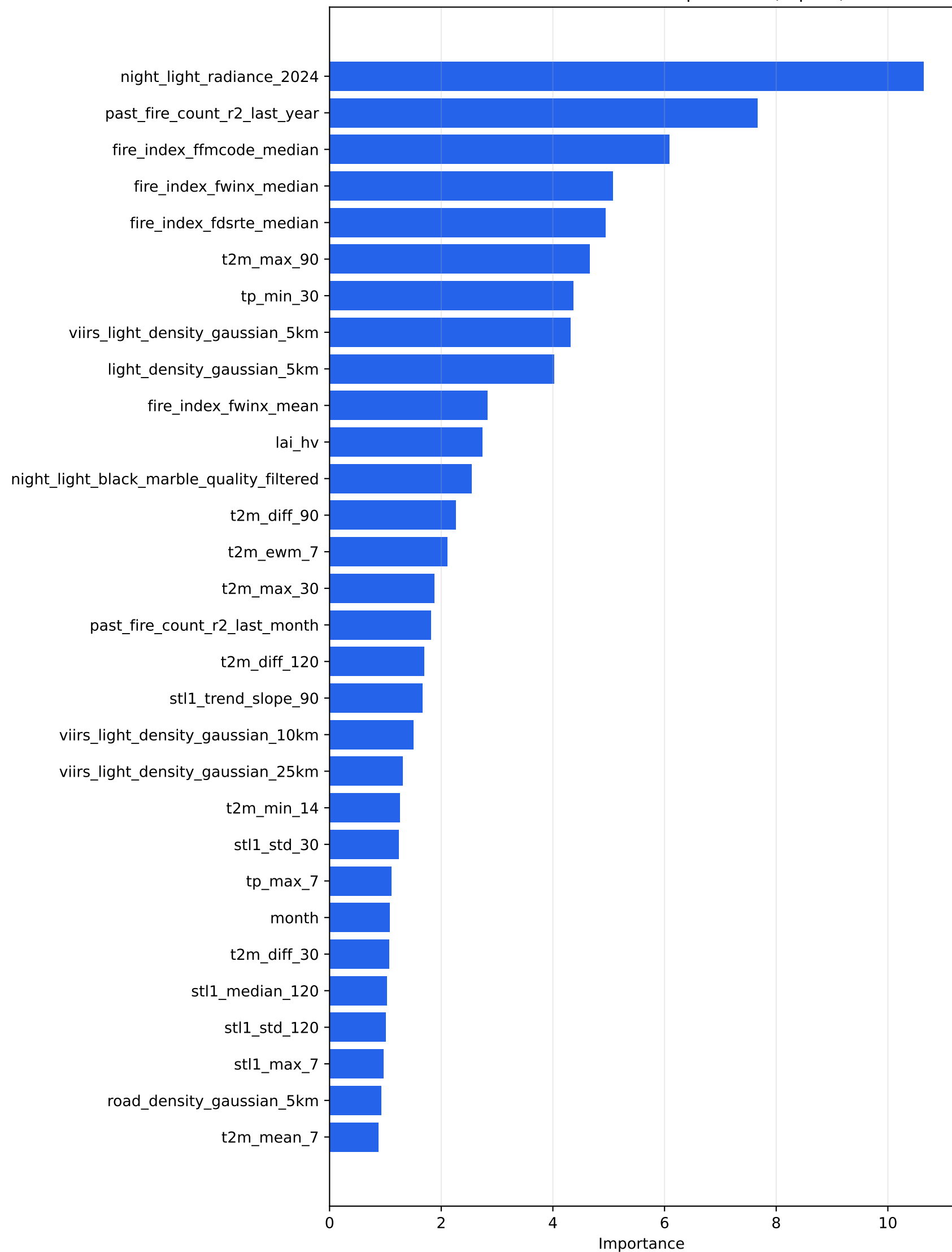
Native CatBoost Feature Importance (Top 30)
