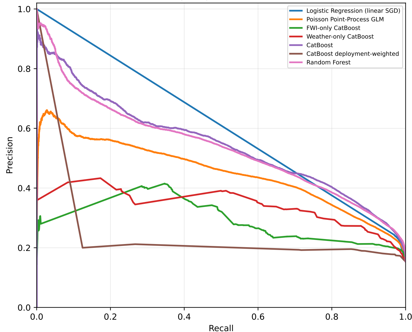
Global sampled precision-recall curves
