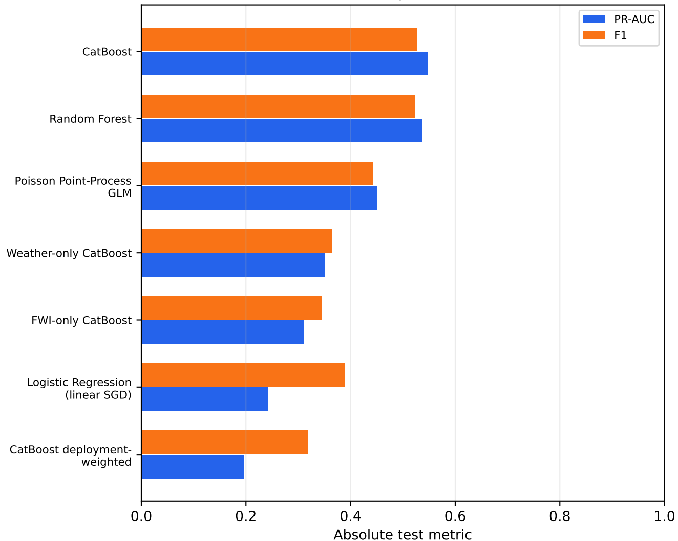
Global sampled metrics
