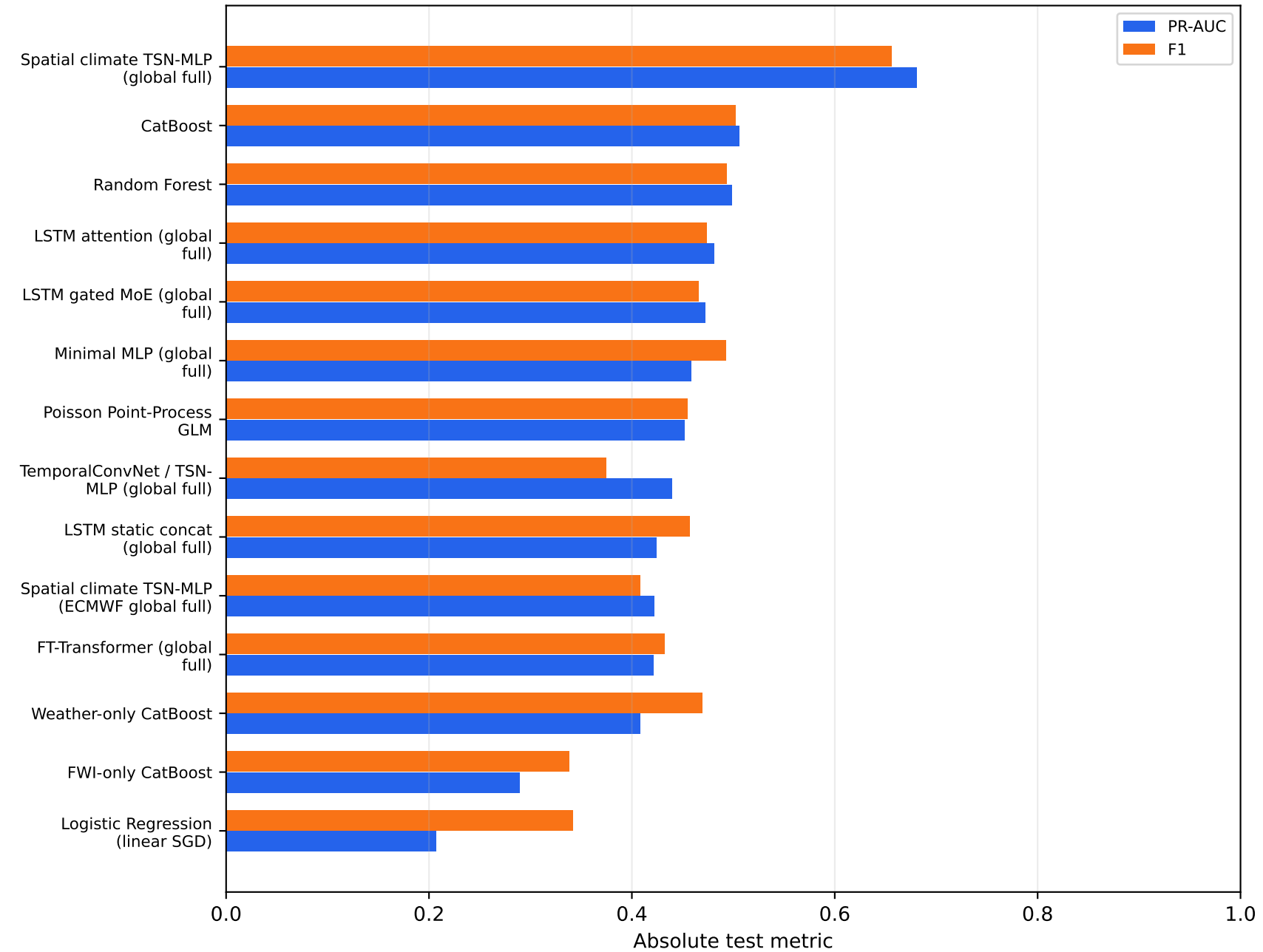
Global sampled metrics
