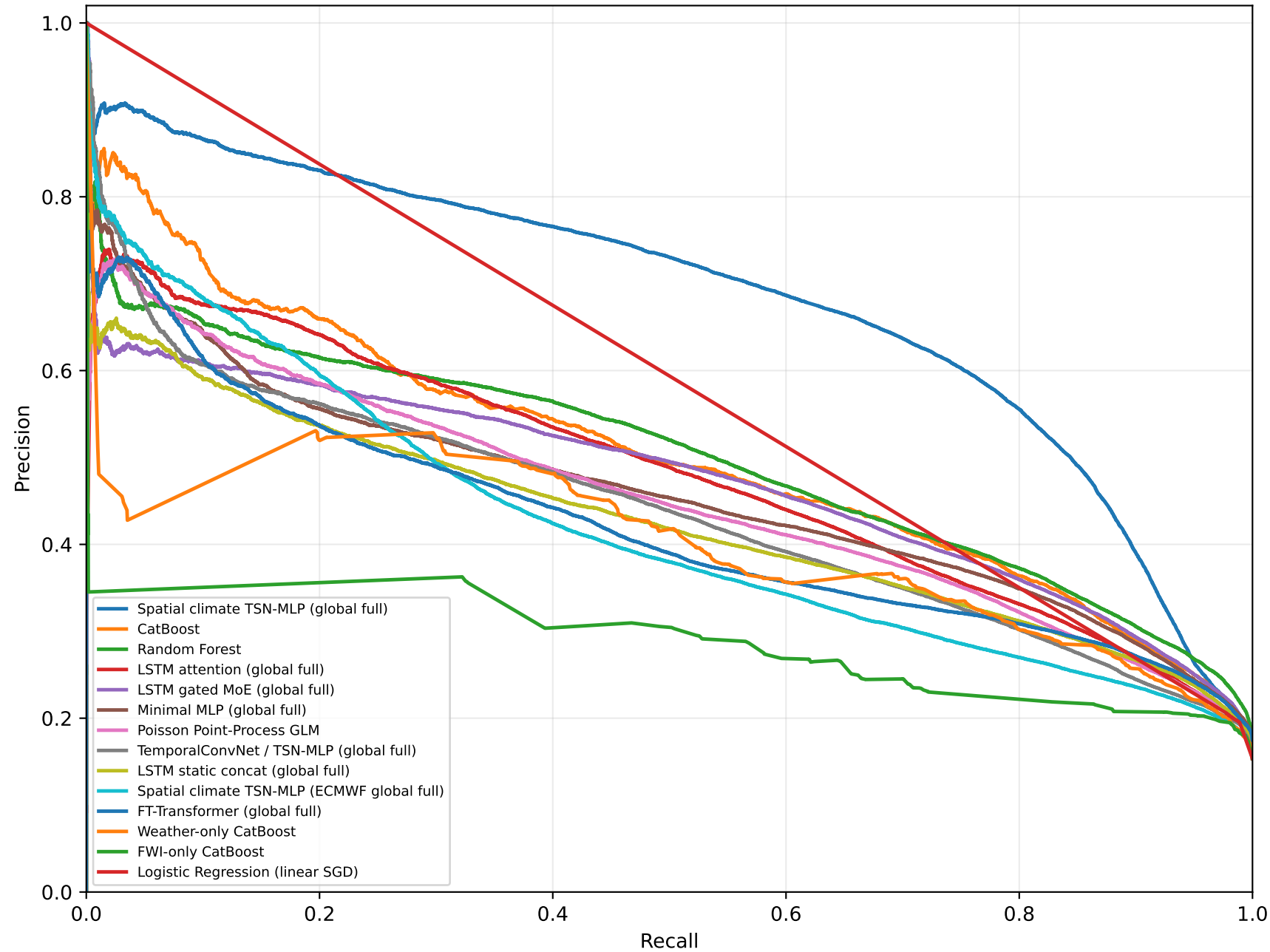
Global sampled precision-recall curves
