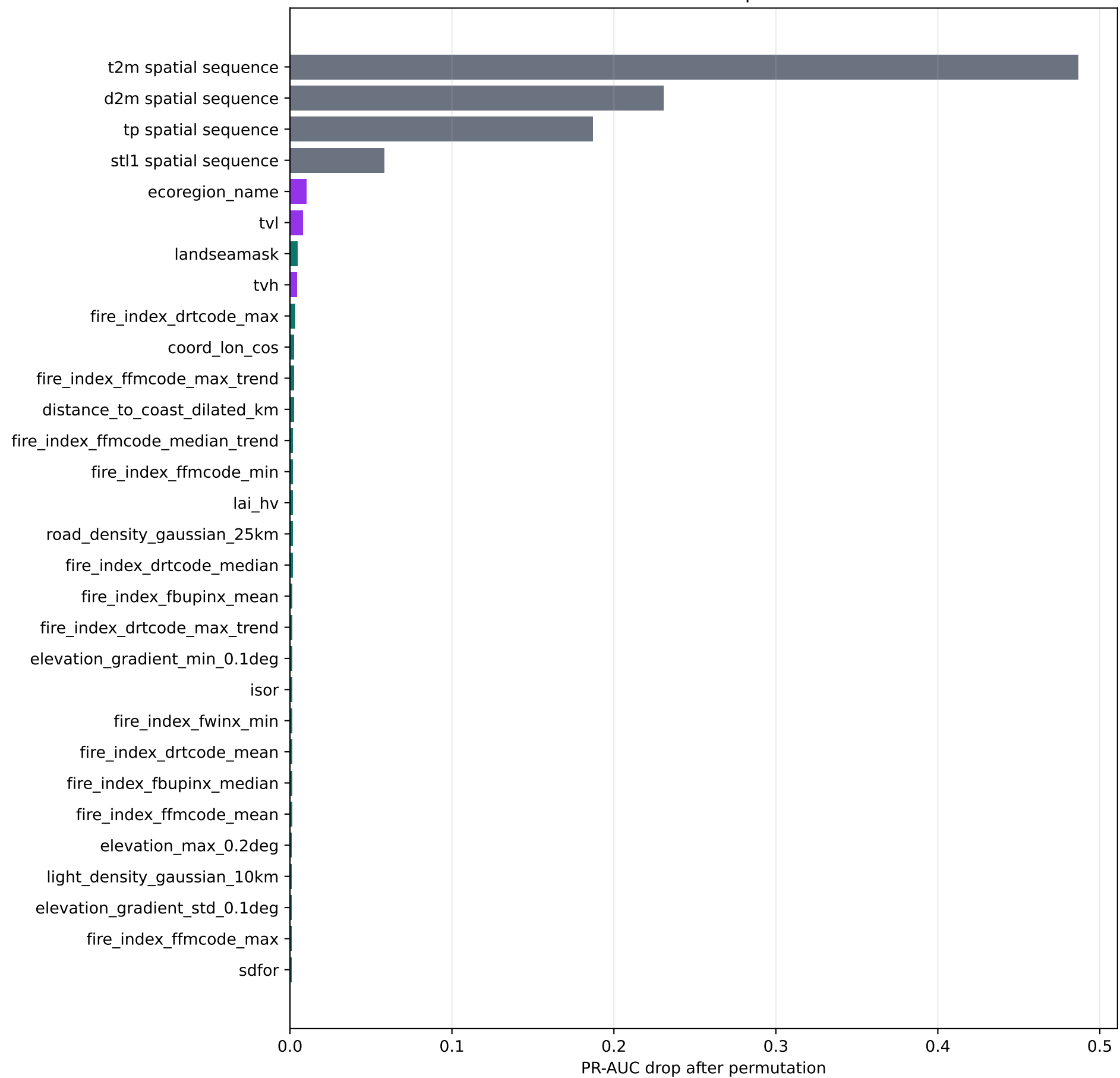
Neural feature importance
