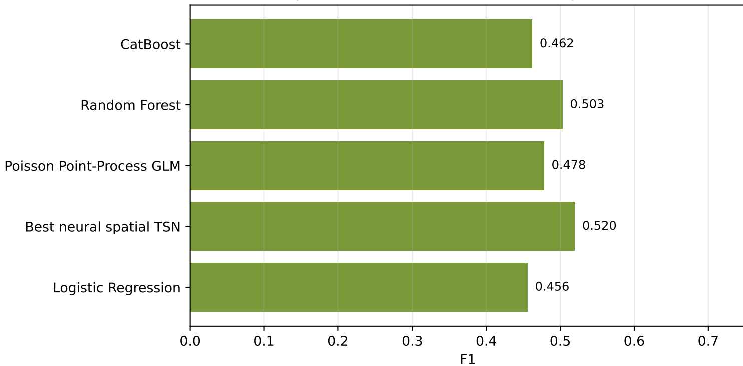
Representative ERA5 -> ECMWF no-tp model F1
