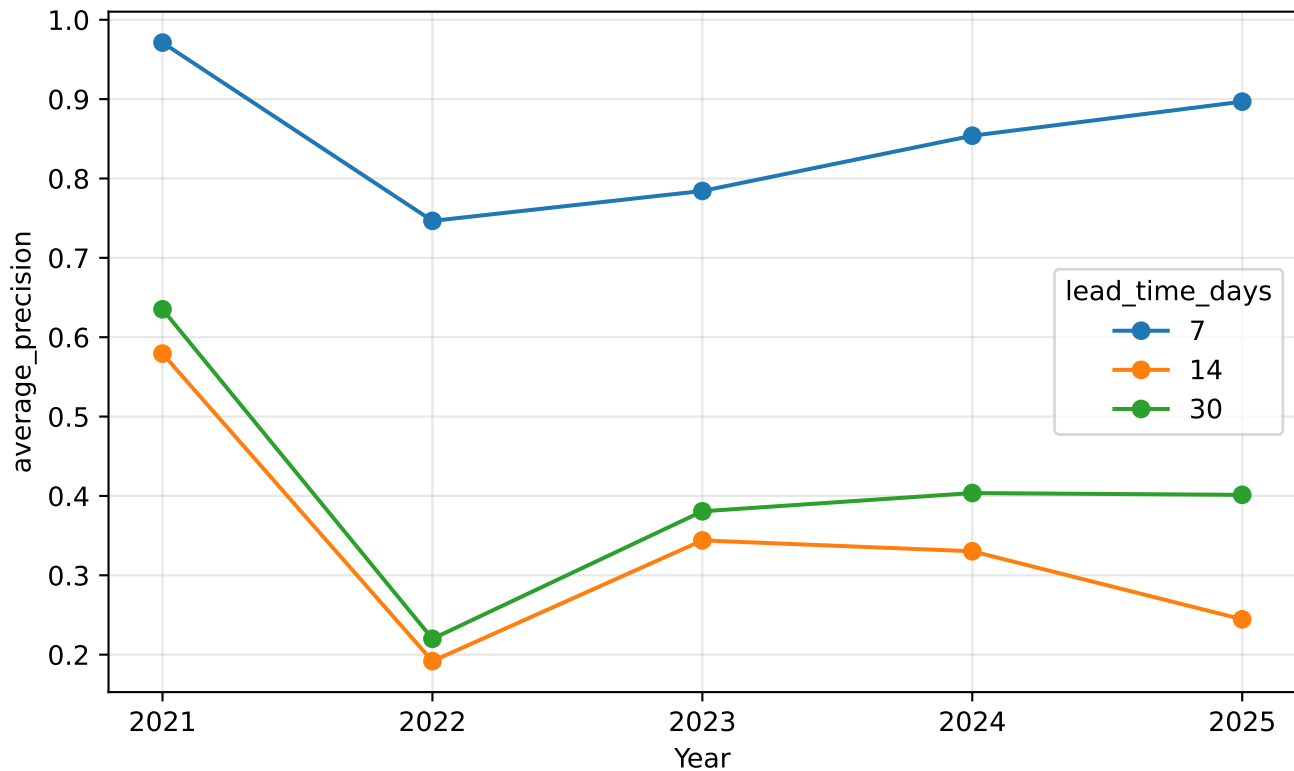
Lead-Time PR-AUC
