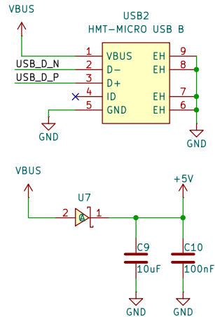
MICRO USB B
