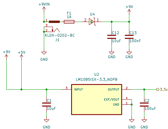
Voltage Regulator
