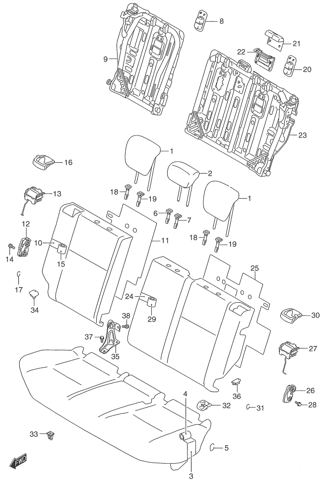
ZC33S 871A REAR SEAT
