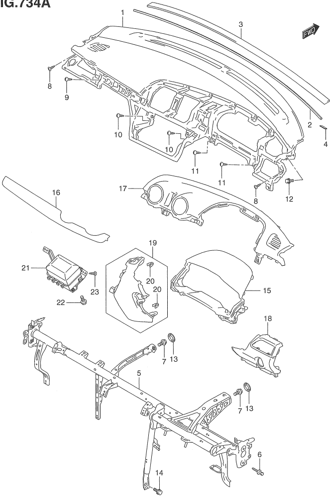
ZC33S 734A INSTRUMENT PANEL UPPER
