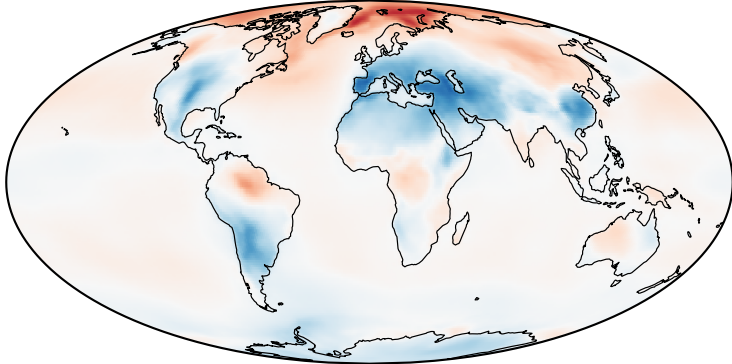
b EC-Earth3
