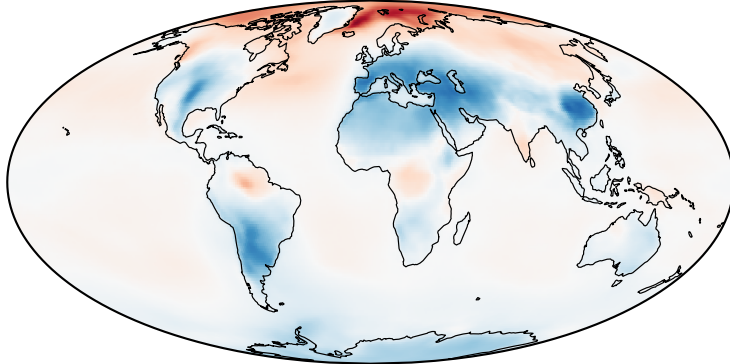
c EC-Earth3-AerChem
