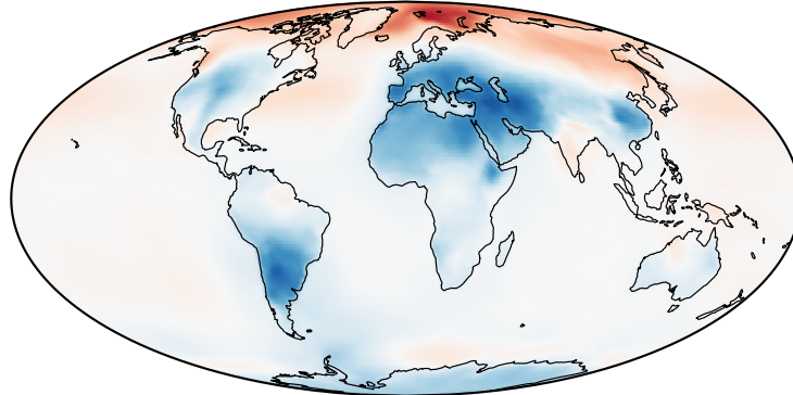
h GFDL-CM4
