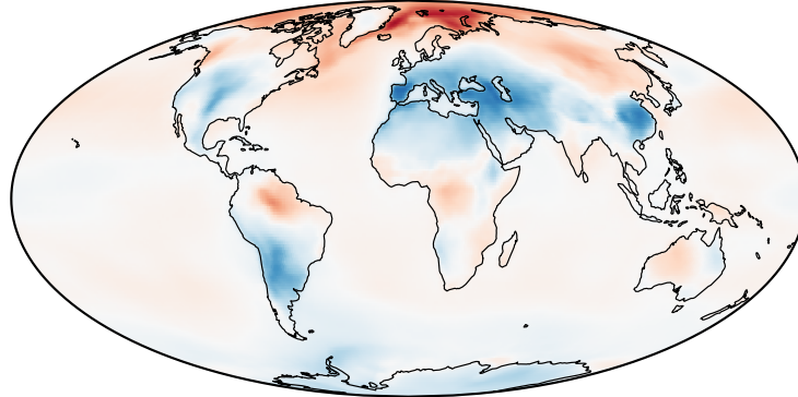
d EC-Earth3-CC
