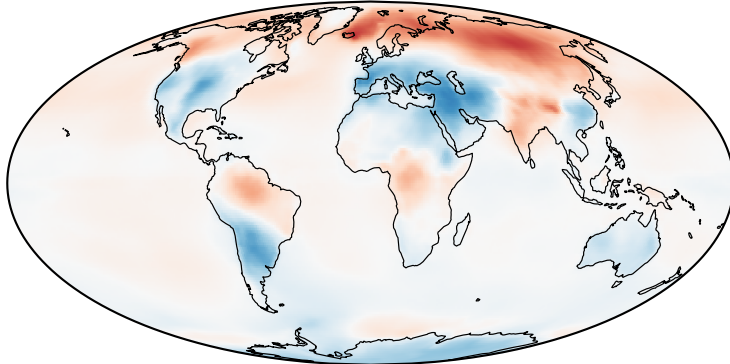
g FGOALS-g3
