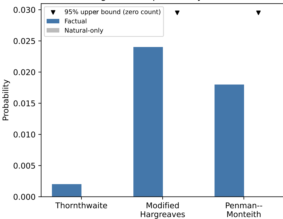
c GCMagicc event probability, 2021--2025
