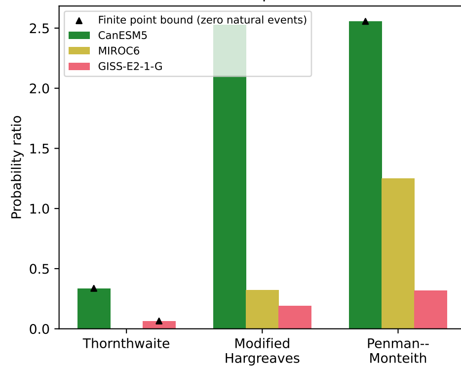
d CMIP6 SMILE comparison, 1995--2014
