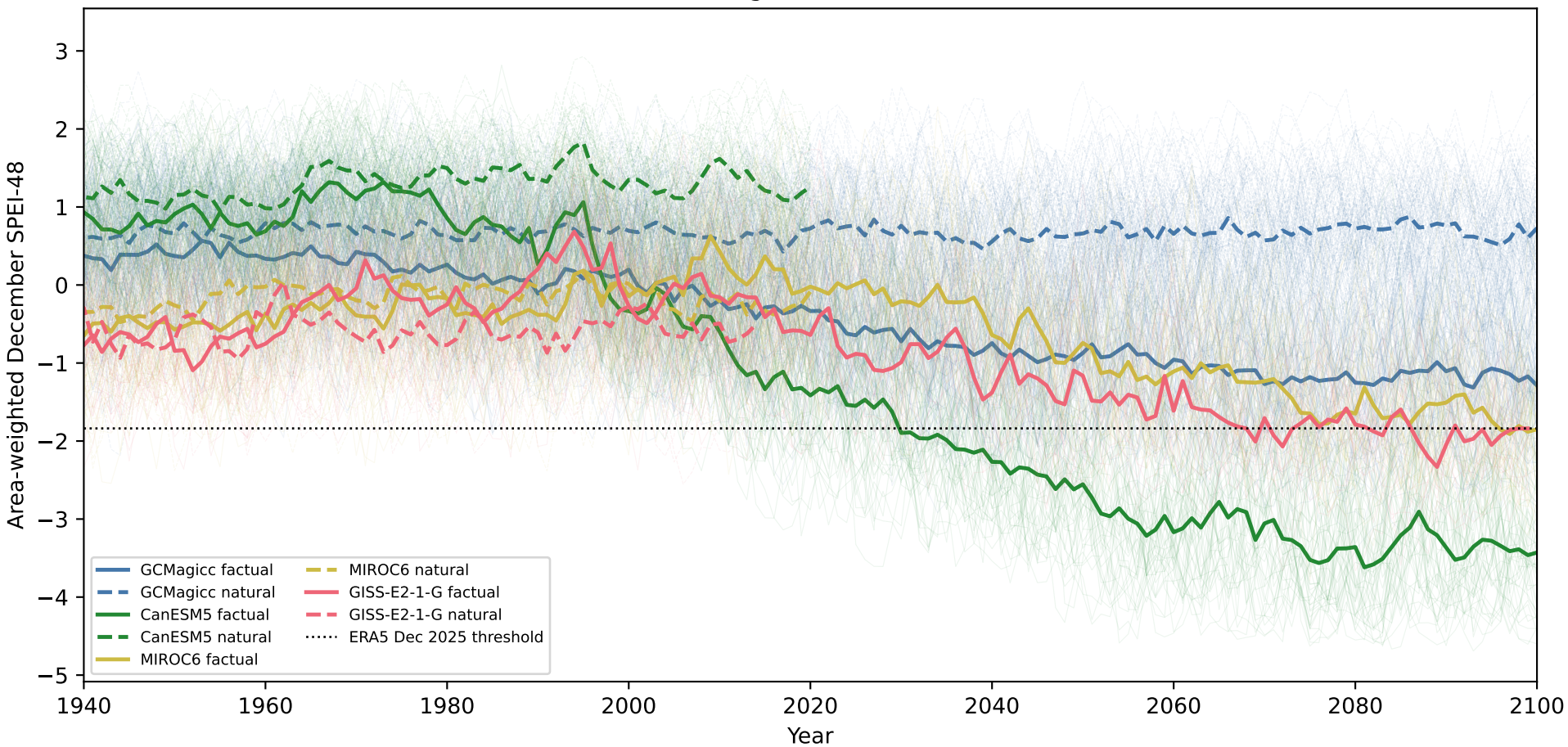
Iran SPEI-48: GCMagicc and three CMIP6 SMILES
