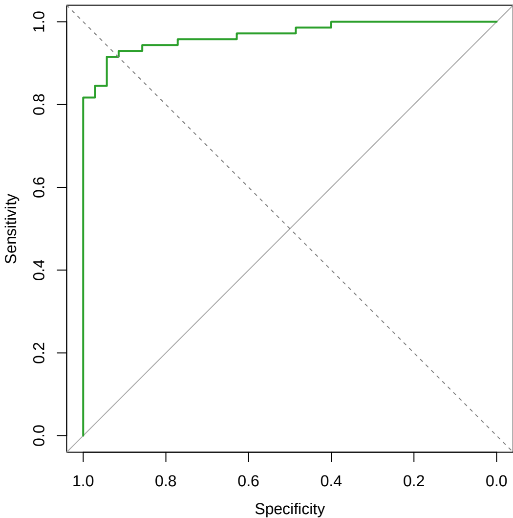
Development Apparent ROC (AUC = 0.968)
