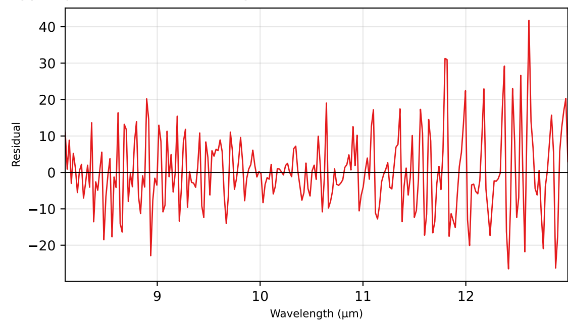
Per-pixel radiance fit & residual (Hyperspectral w/ downwelling)
