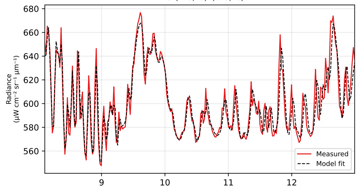
Per-pixel radiance fit & residual (Hyperspectral w/ downwelling)
