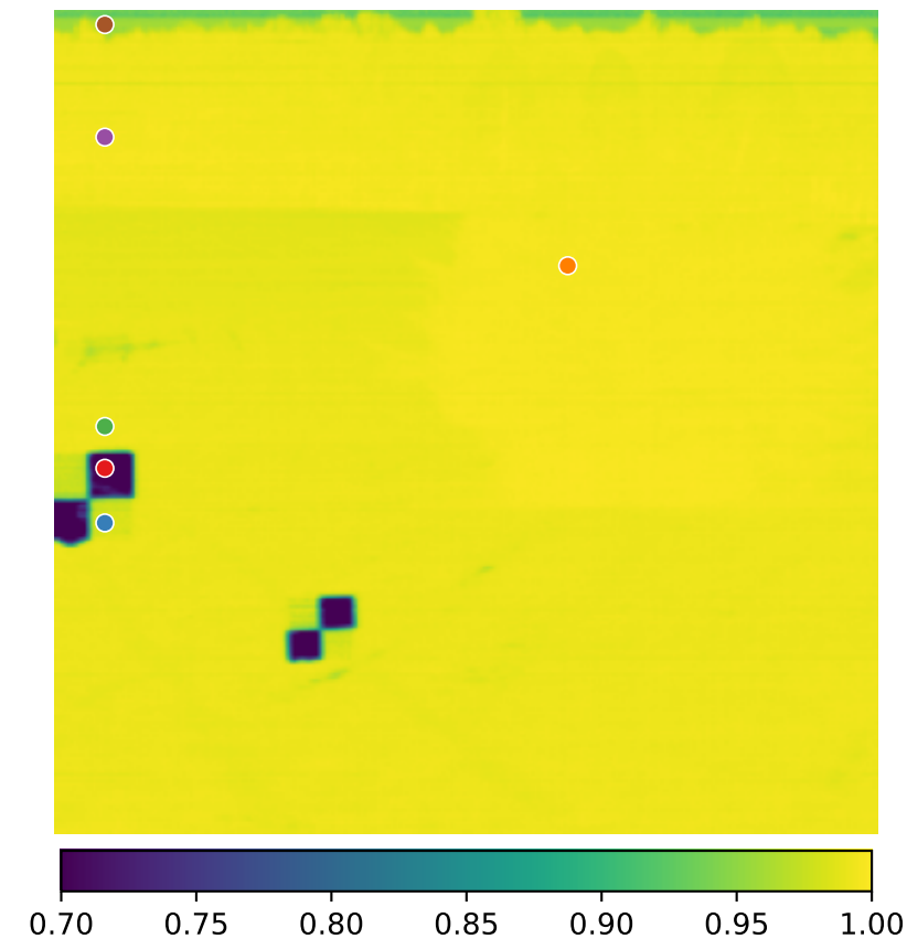
Mean emissivity no dw
