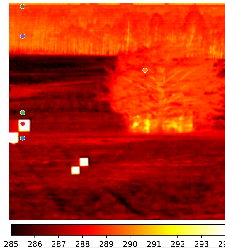
Temperature no dw (K)
