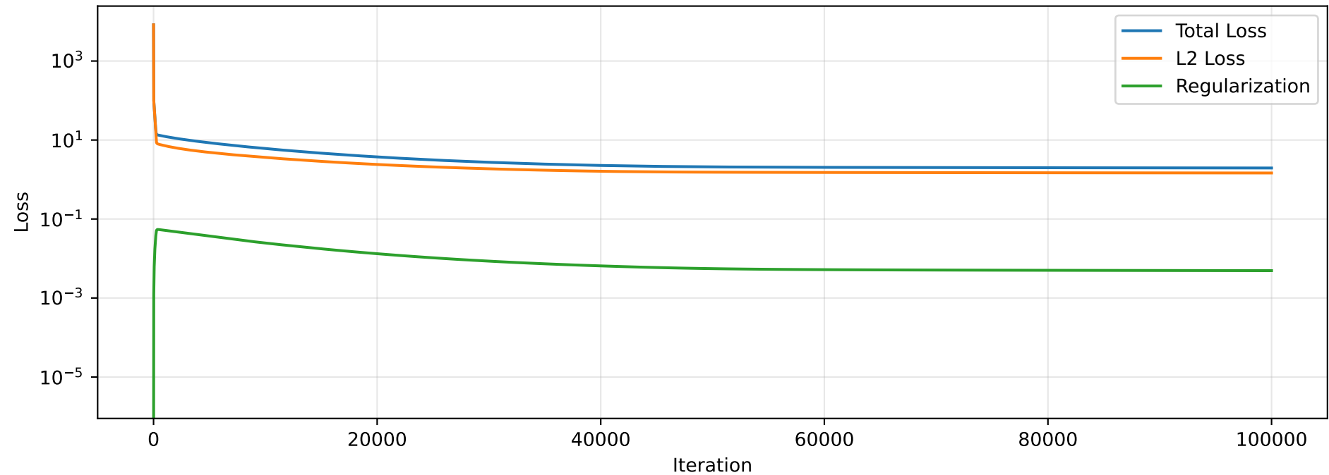
Training Loss
