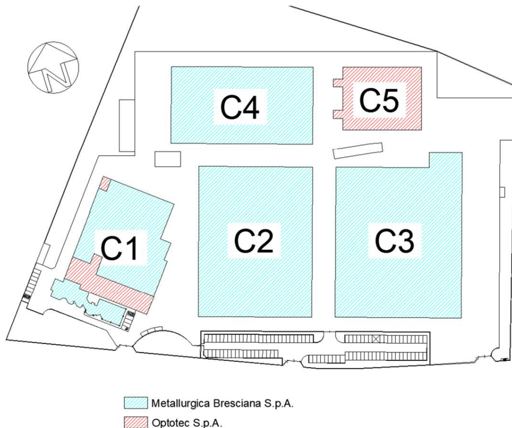
General plan of the production unit with identification of the 5 different factory buildings and the areas used by the companies Metallurgica Bresciana and Optotec
