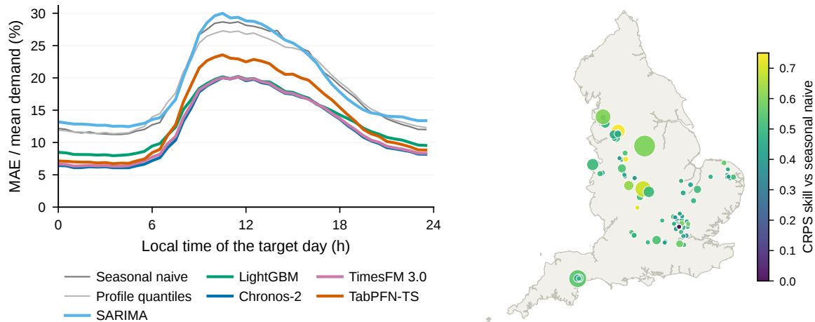
Figure 3: Left: normalised error by local time of the target day for the models without covariates and the baselines. Right: CRPS skill of Chronos-2 with forecast weather at each site, with marker area proportional to mean demand.
