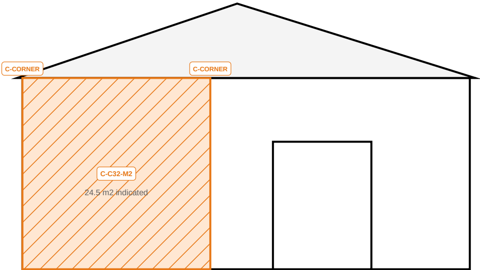
NORTH ELEVATION
