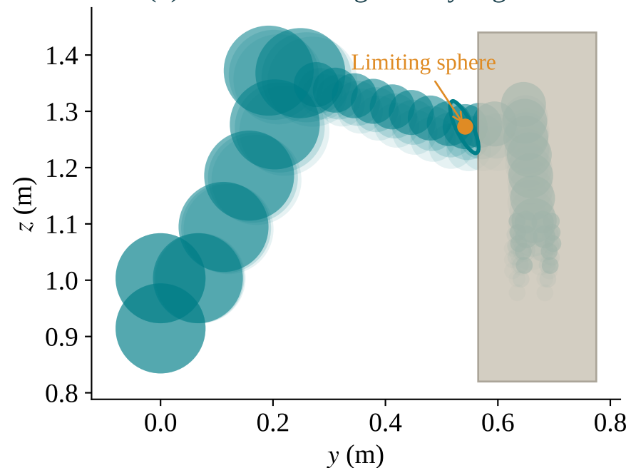
(b) UR5 collision geometry + ghosts
