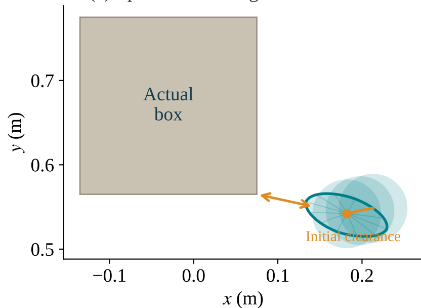
(c) Sphere motion against the obstacle
