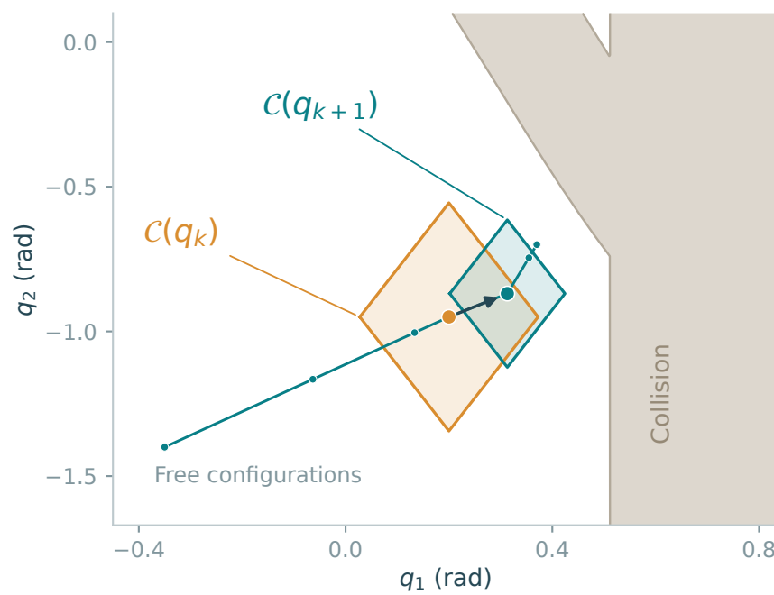
(c) Certificates in configuration space
