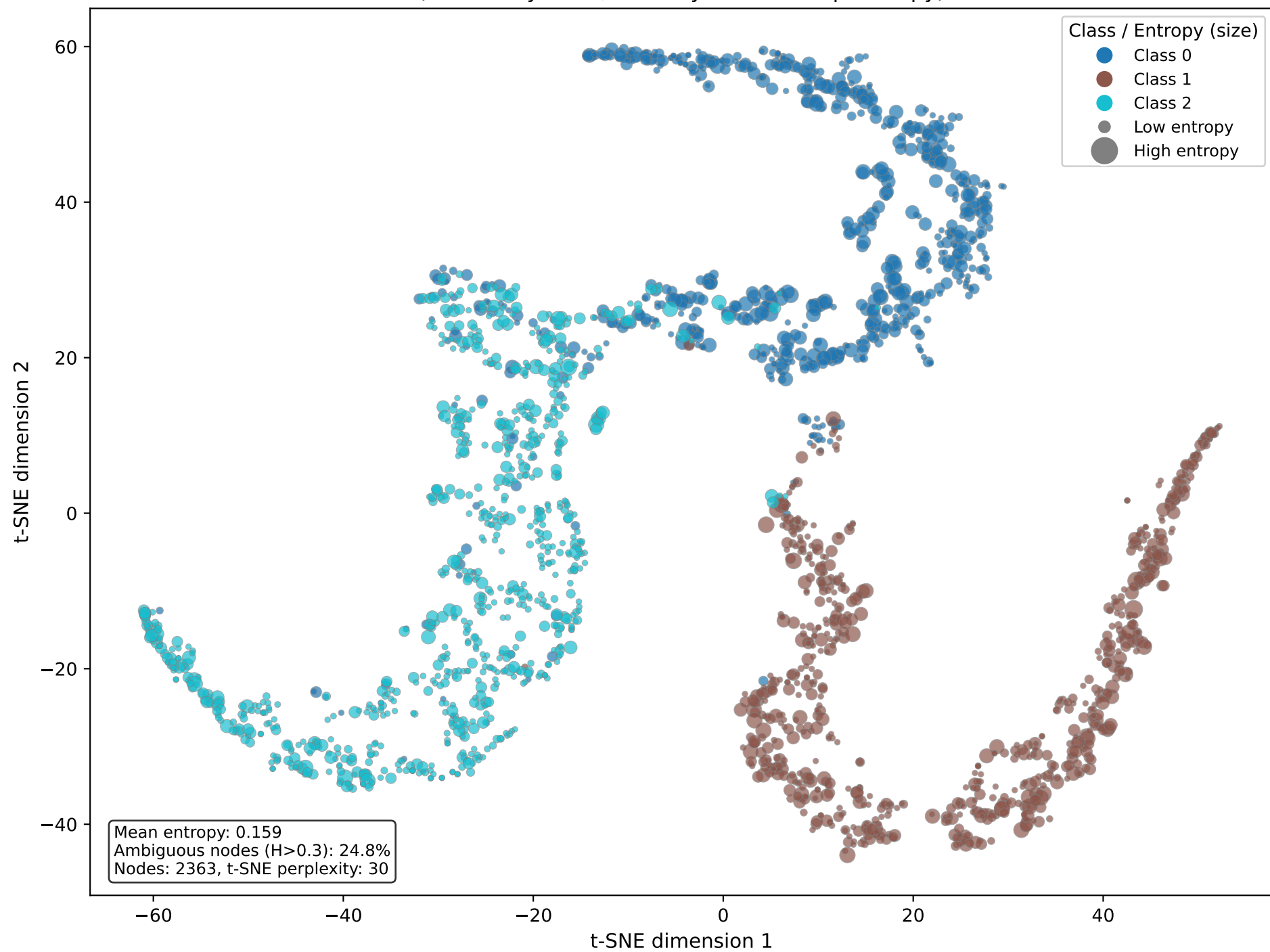
t-SNE Visualization of GCN Embeddings — ACM (colored by class, sized by membership entropy)
