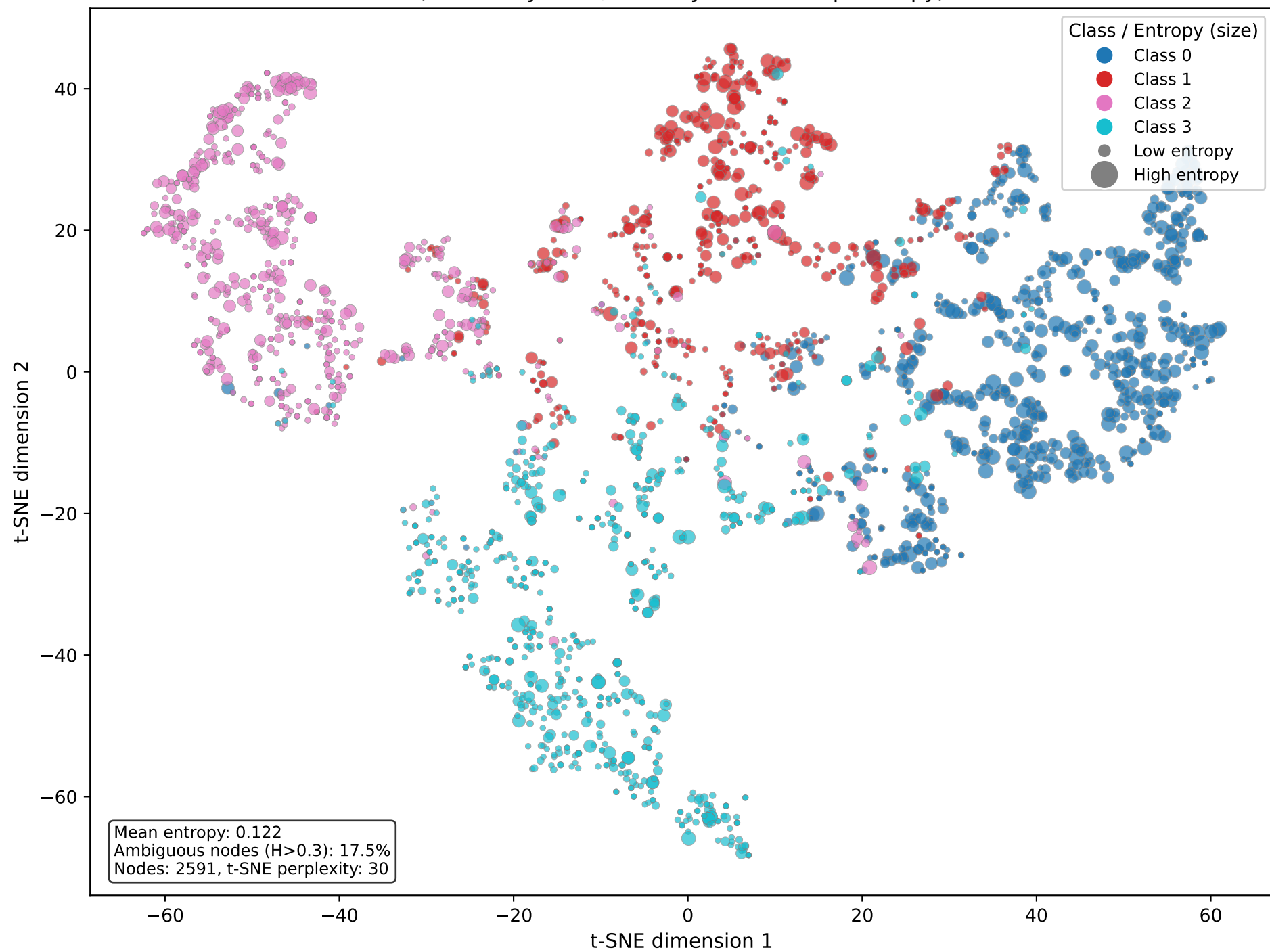
t-SNE Visualization of GCN Embeddings — DBLP (colored by class, sized by membership entropy)
