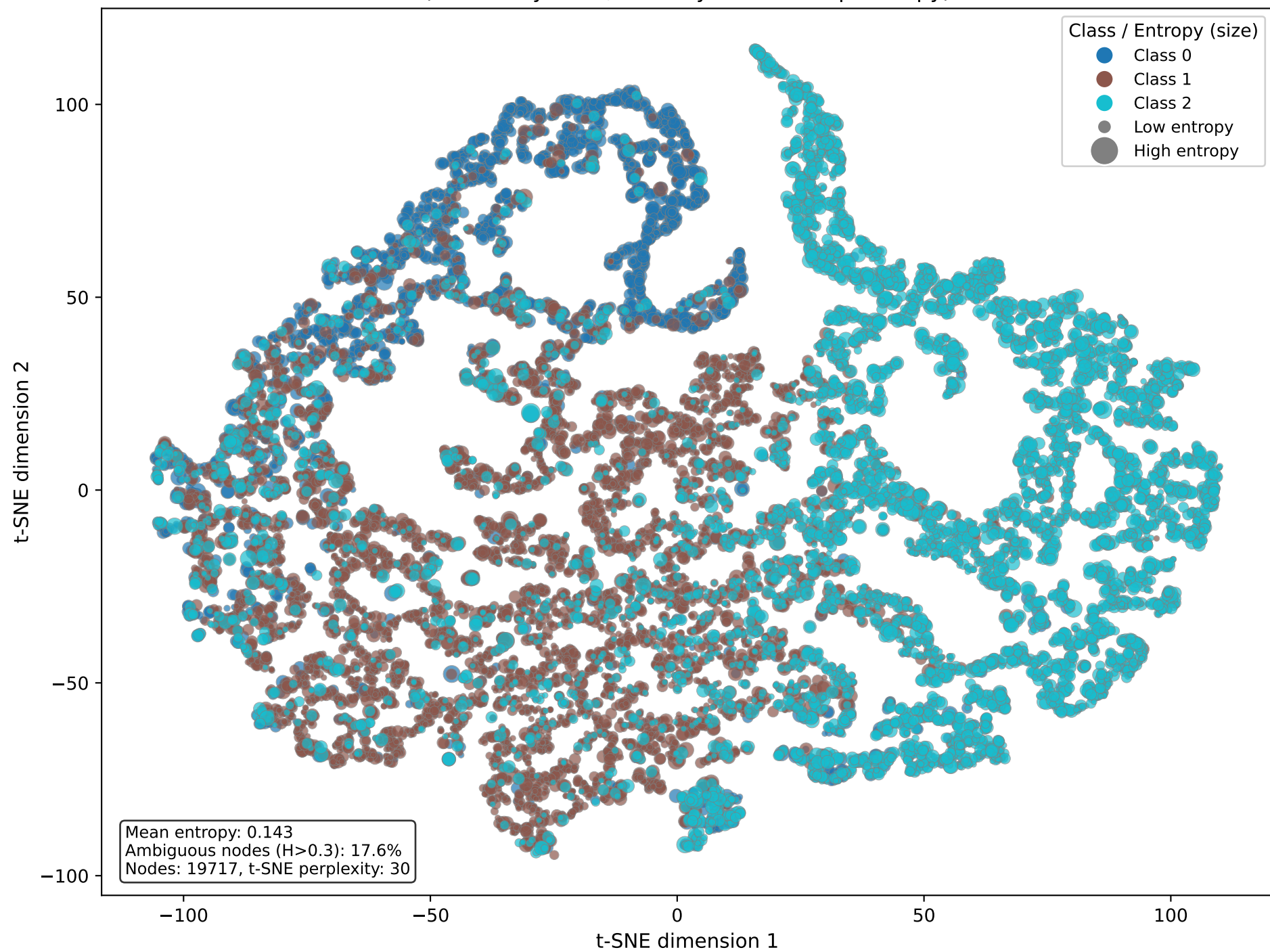
t-SNE Visualization of GCN Embeddings — PubMed (colored by class, sized by membership entropy)
