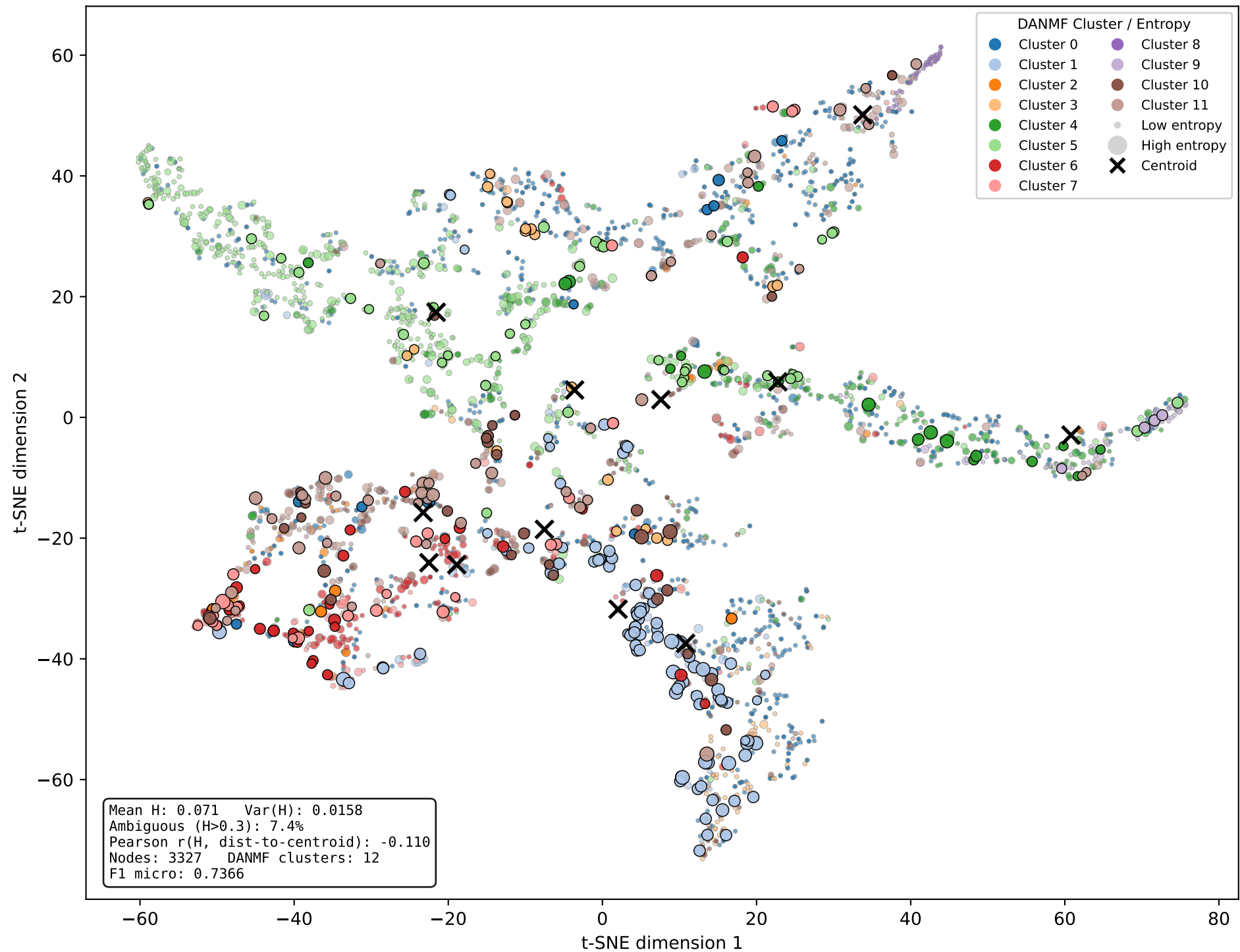
t-SNE of GCN Embeddings Coloured by DANMF Cluster -- CiteSeer
