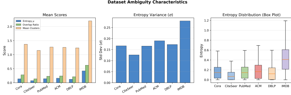
Figure 7: Dataset ambiguity characteristics. (Left) Mean entropy, overlap ratio, and cluster count per dataset. IMDB stands out with the highest entropy and overlap ratio. (Center) Entropy standard deviation. (Right) Entropy distribution box plots. IMDB shows the widest distribution, explaining why it benefits most from adaptive thresholding.
